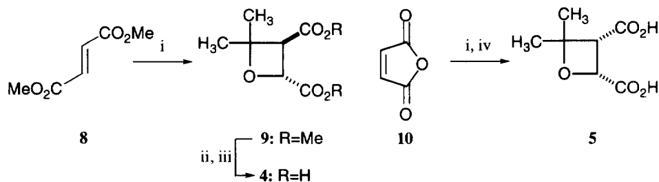
Scheme 4. Reagents: i, h\nu , acetone ; ii, LiOH; iii, Dowex 50W-X2 ( \text{H}^+ ); iv, \text{H}_2\text{O}
