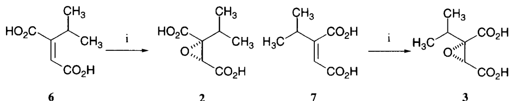
Scheme 3. Reagents: i, \text{H}_2\text{O}_2 , \text{Na}_2\text{WO}_4 \cdot 2\text{H}_2\text{O} , \text{NaOH}
