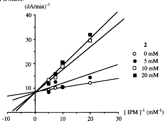
Fig. 1. Lineweaver-Burk plot of the effect of the oxirane 2 on IPMDH reaction.
